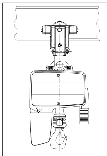
Duwloopkat
