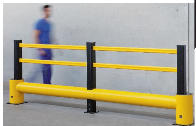
Basic and extension sets with rails and sign holder (accessories)
