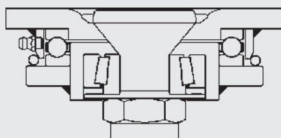
Swivel fork head
