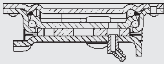
Swivel bearing
