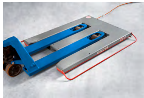
E-shape with standardised recesses for pallet trucks or drawbar stackers
