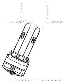
Accessible passageway width: 2210 mm for 800 x 1200 mm pallets, lengthwise entry
