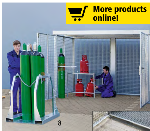
Container with roof and double doors – gas cylinder pallet/shelf/holder as accessories
