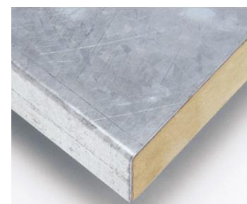
Sheet steel cladding – 2 mm thick, hot dip galvanised, curved up at front and rear, resistant to impact, oils, greases, liquids
