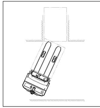
Accessible passageway width: 2210 mm for 800 x 1200 mm pallets, lengthwise entry
