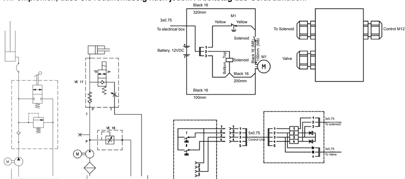
Hydraulikplan
