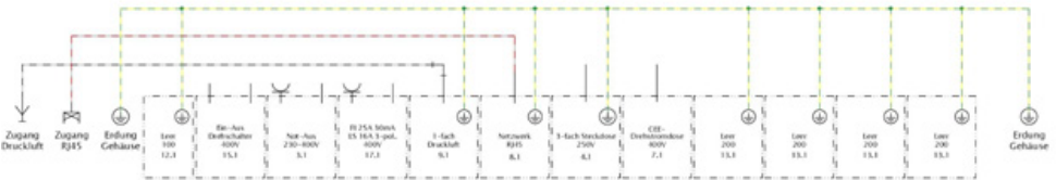
Referensplan 400V
