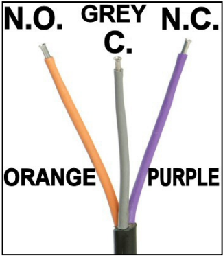
Figure 5 - Contact configuration, signalling cable
