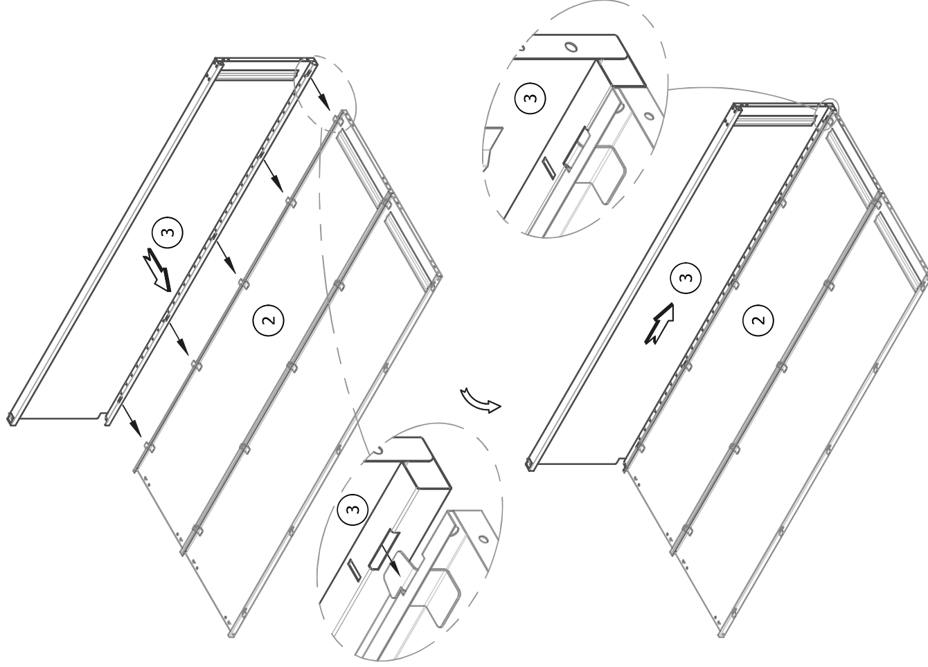
Step: 2.1 RH Side Panel Joining
