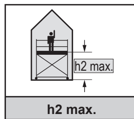
Maximum permitted height of working platform inside of buildings
