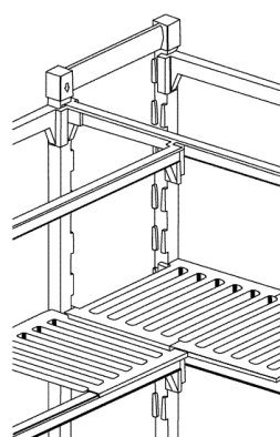
MOUNT TRAVERSES
