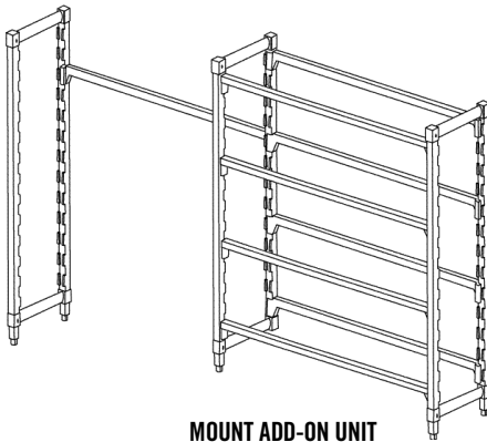
MOUNT ADD-ON UNIT
