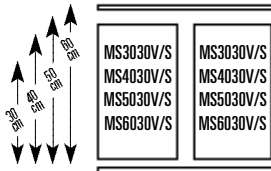
Shelf Configuration for 90 cm Traverse.
