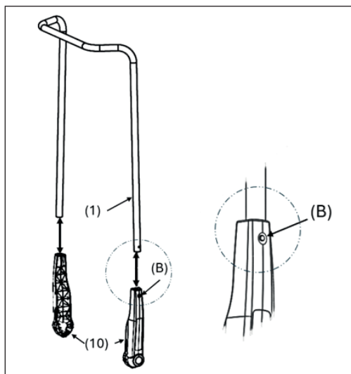
Fig. 8: Fitting the handle fittings
