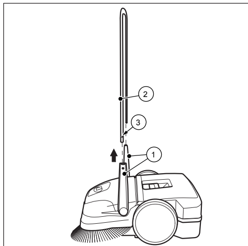
Fig. 13: Sliding bracket disassembly (not starmix 497)
