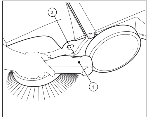
Fig. 14: Sliding bracket disassembly (not haaga 375)
