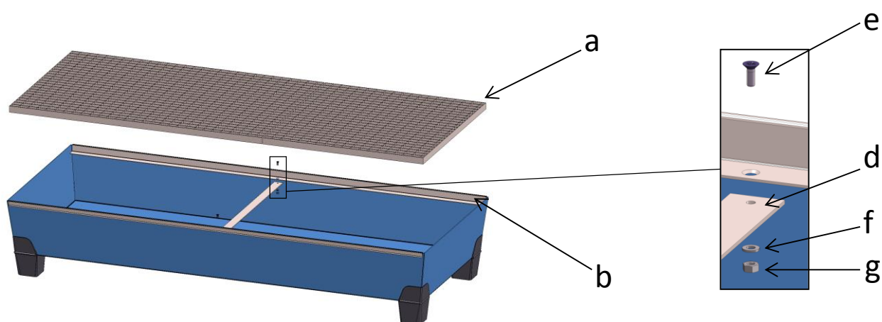
Fig. 3.3-2: sump type 5
