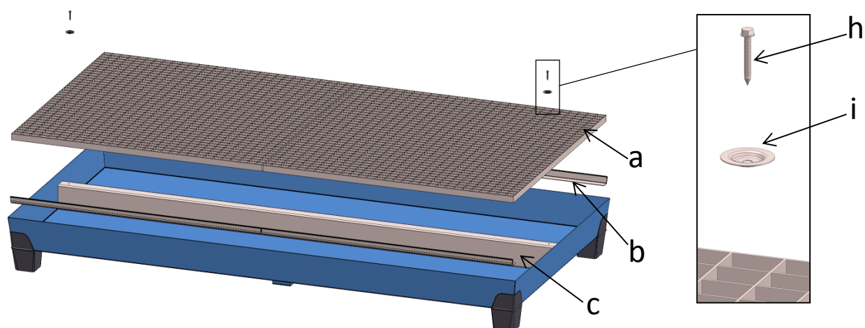
Fig. 3.3-3: sump type 7
